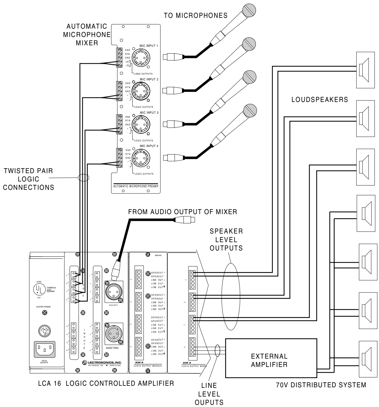
Figure 13 - Interconnection Diagram
