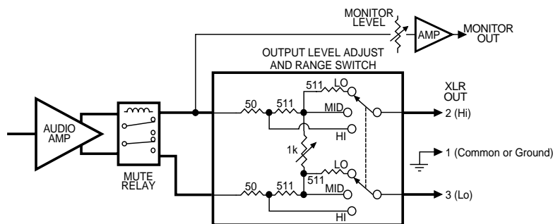
UCR200D Simplified Audio Output Circuit
