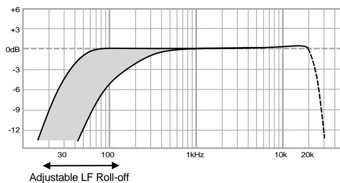
Typical System Frequency Response
